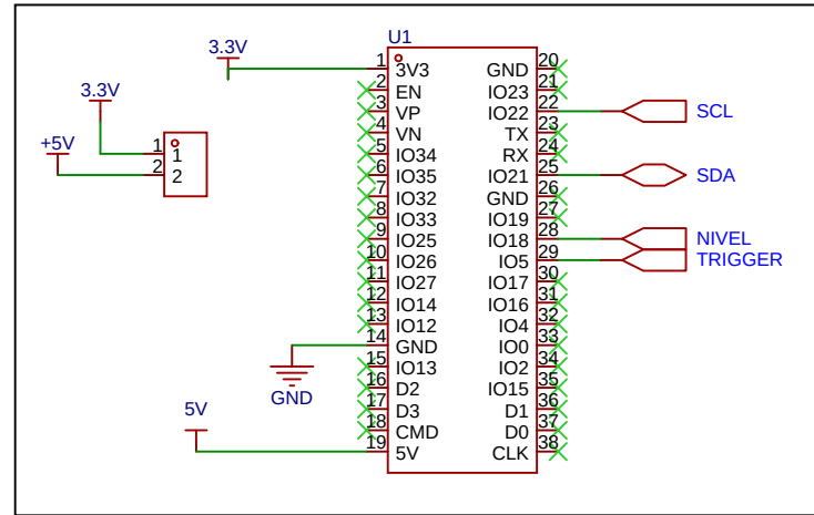
ESP32-DevKitC
